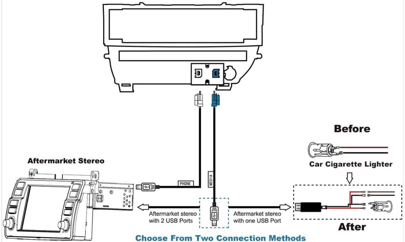
Figure 3: Wiring diagram illustrating the connections for the aftermarket stereo and the integrated USB ports. Note the two connection methods for aftermarket stereos (with 2 USB ports or 1 USB port).
