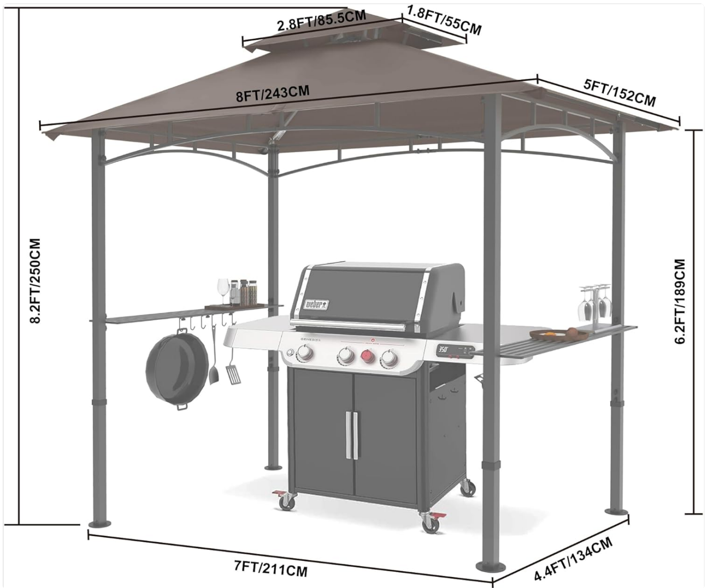
Figure 2: Key dimensions of the grill gazebo.
