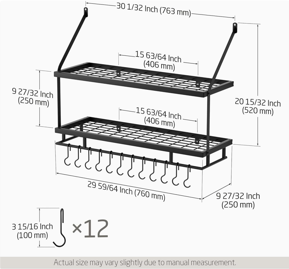
Image: Detailed dimensional drawing of the pot rack, including shelf depth, width, and overall height, along with hook dimensions.
