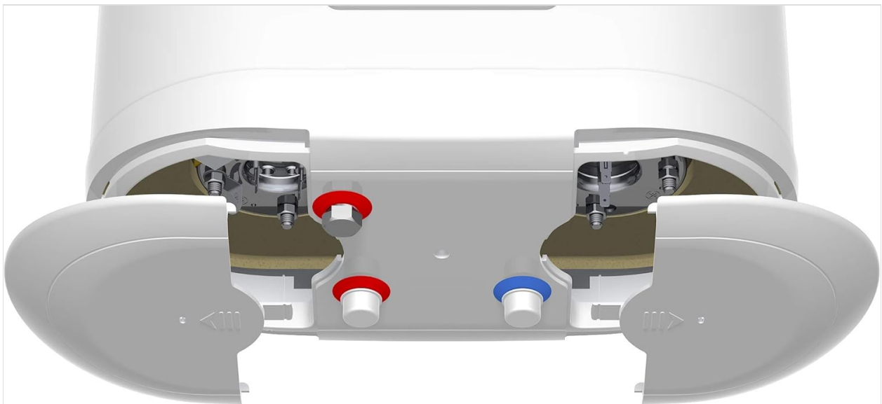
Figure 3.1: Close-up view of the water inlet (blue) and outlet (red) connections at the base of the boiler. The safety valve should be installed on the blue inlet.
