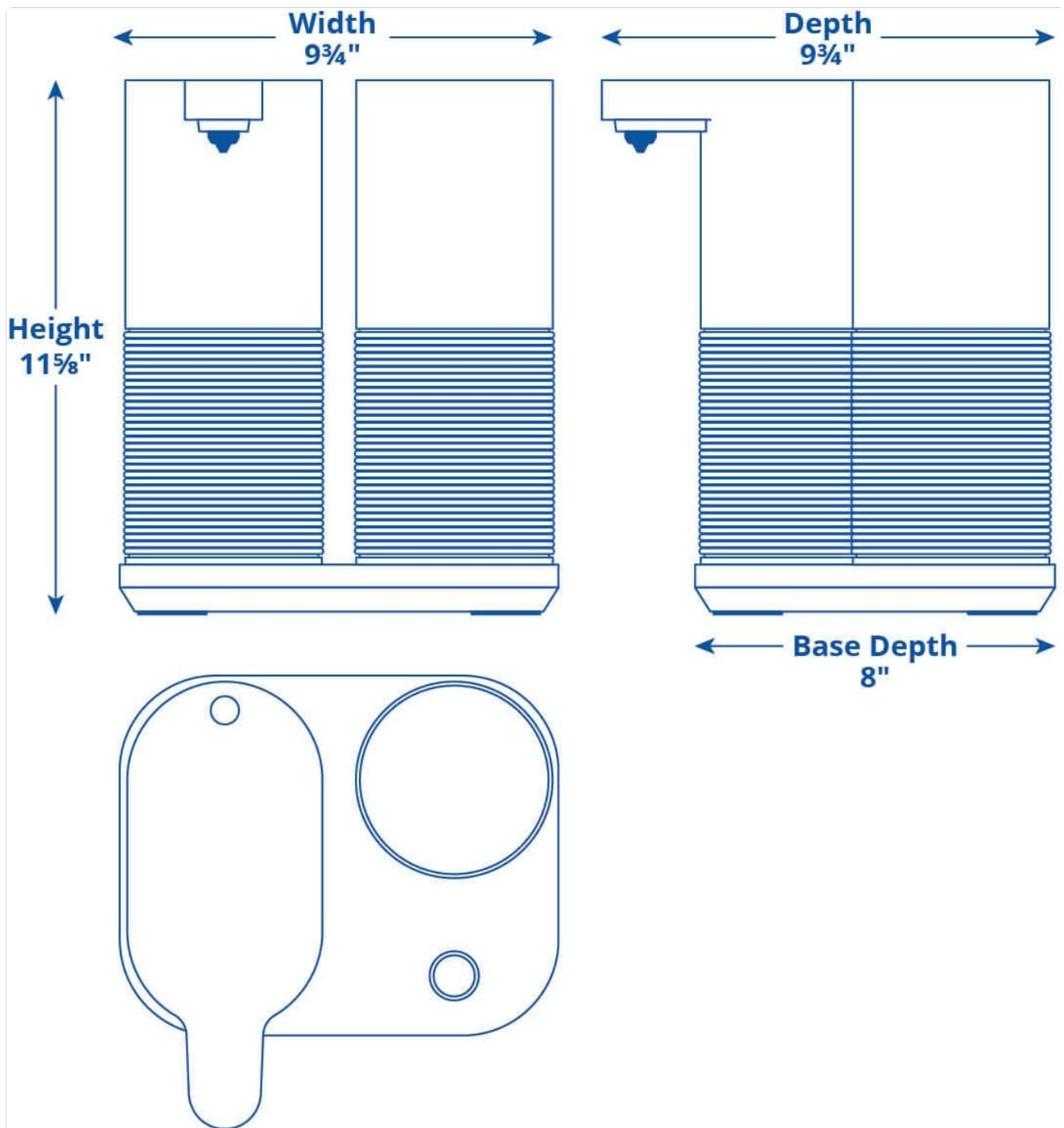
Image 6.1: Product dimensions for the Aquasana Countertop Water Filter System.
