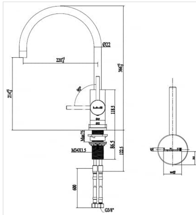
Image: Technical diagram illustrating the dimensions and connection points of the Reginox Spring faucet, including the G 3/8" connectors and mounting details.
