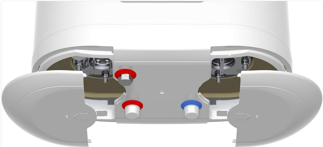
Figure 3: View of the bottom connections, showing the cold water inlet (blue) and hot water outlet (red) pipes, along with the protective covers.
