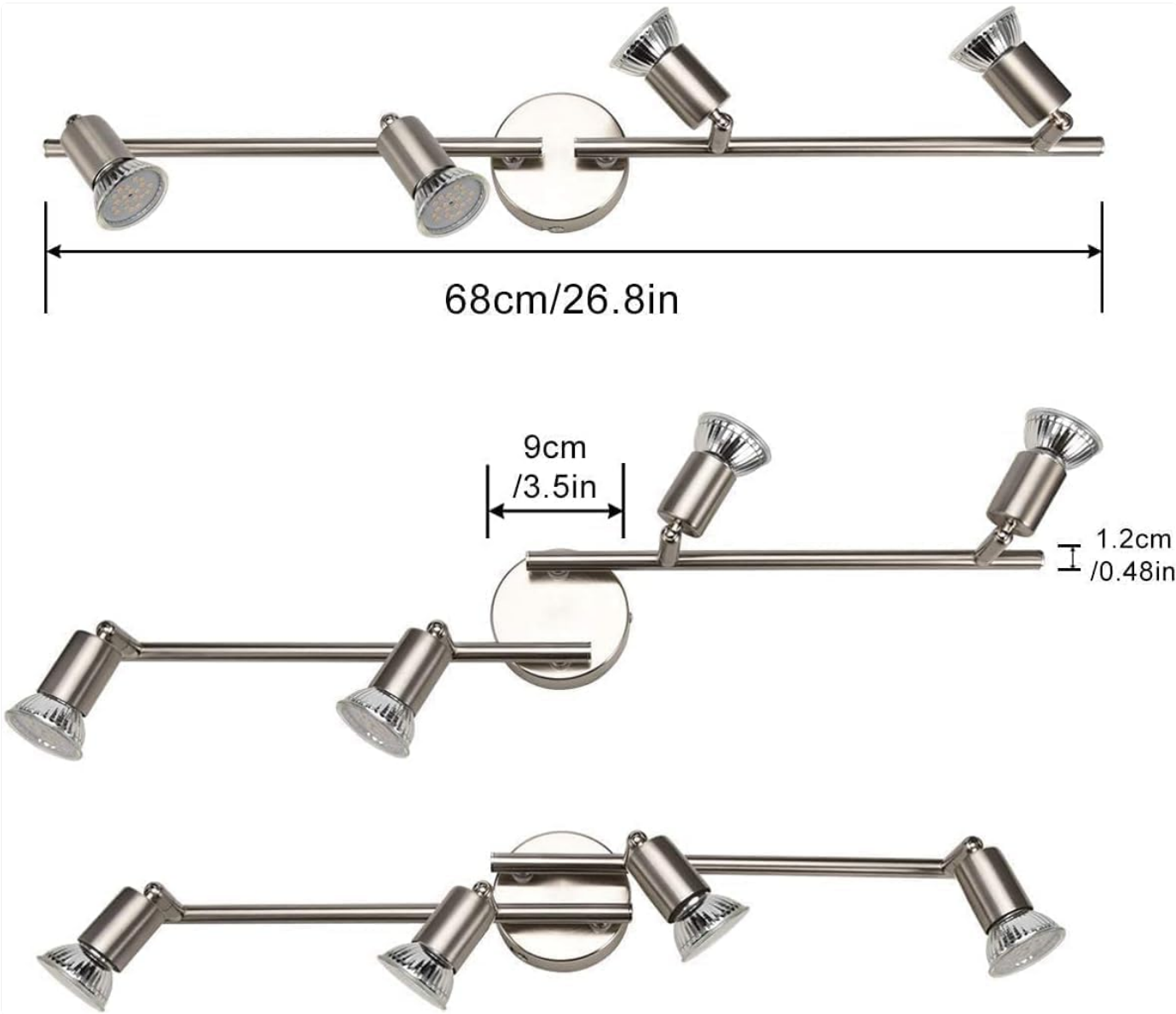
Image 4.1: Detailed dimensions of the wowatt LED Ceiling Light fixture.
