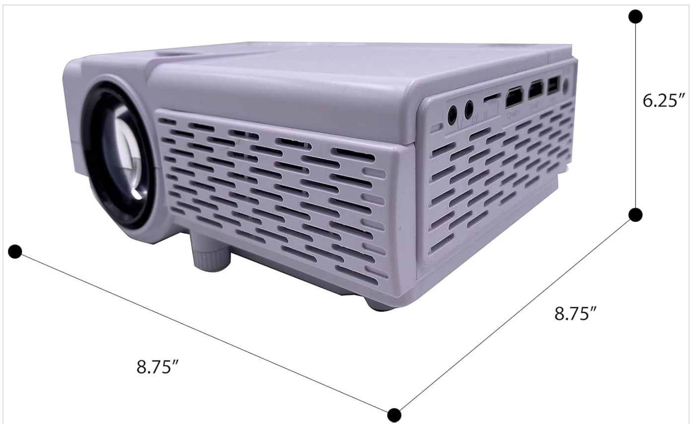
Figure 4.2: Dimensions of the RPJ104 Projector, showing its compact size for portability.
