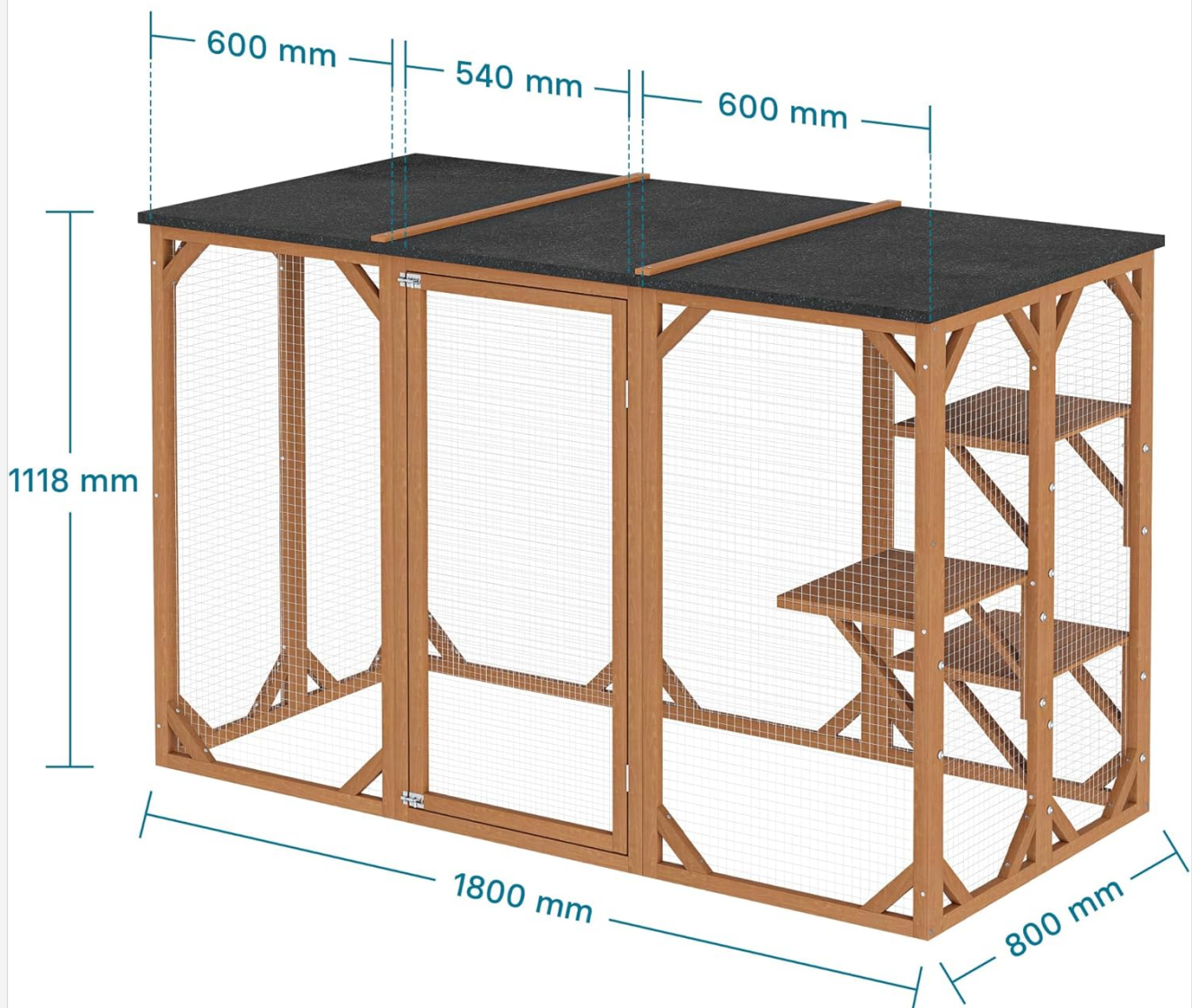
Image 8.1: A diagram illustrating the key dimensions of the Wiltec Cat Outdoor Enclosure XL, including length, width, and height measurements in millimeters.
