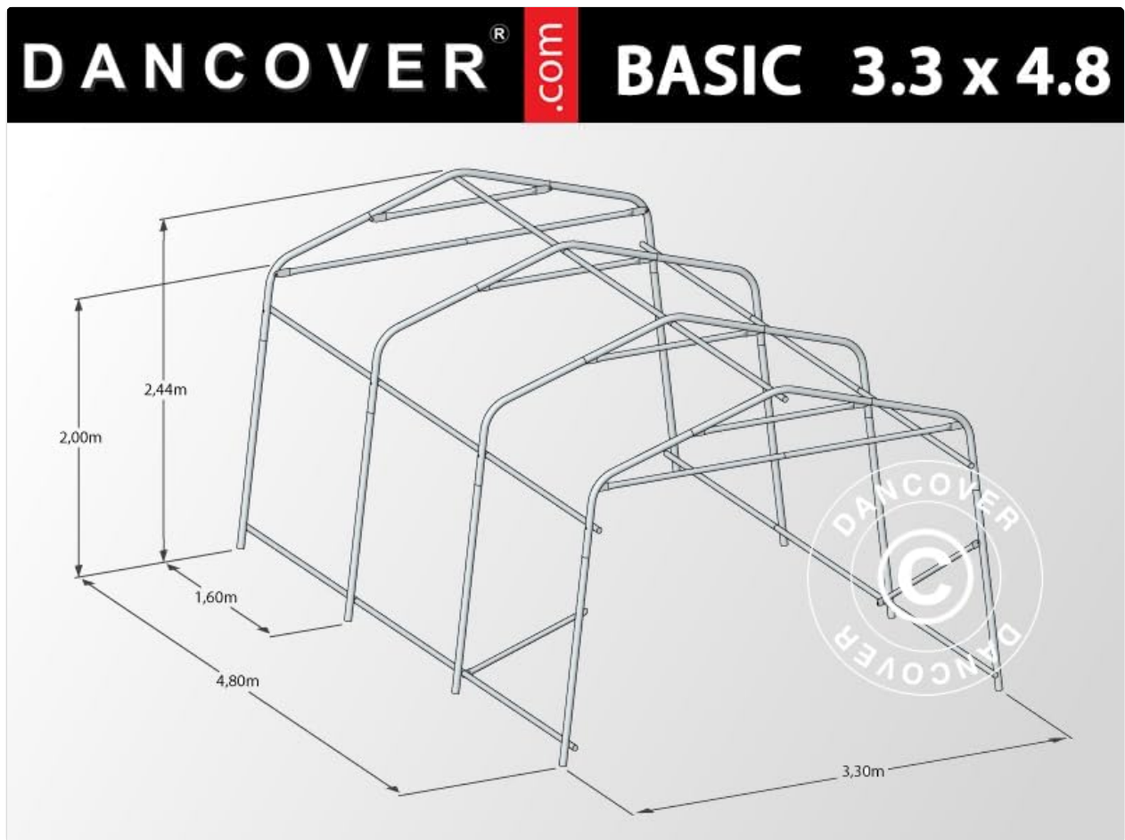
Figure 2: Technical drawing illustrating the frame structure and dimensions (3.30m W x 4.80m L x 2.44m H).
