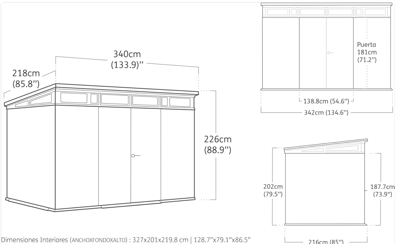
Image: A diagram showing the external dimensions of the Keter Artisan 117 shed, useful for planning placement and assembly.
