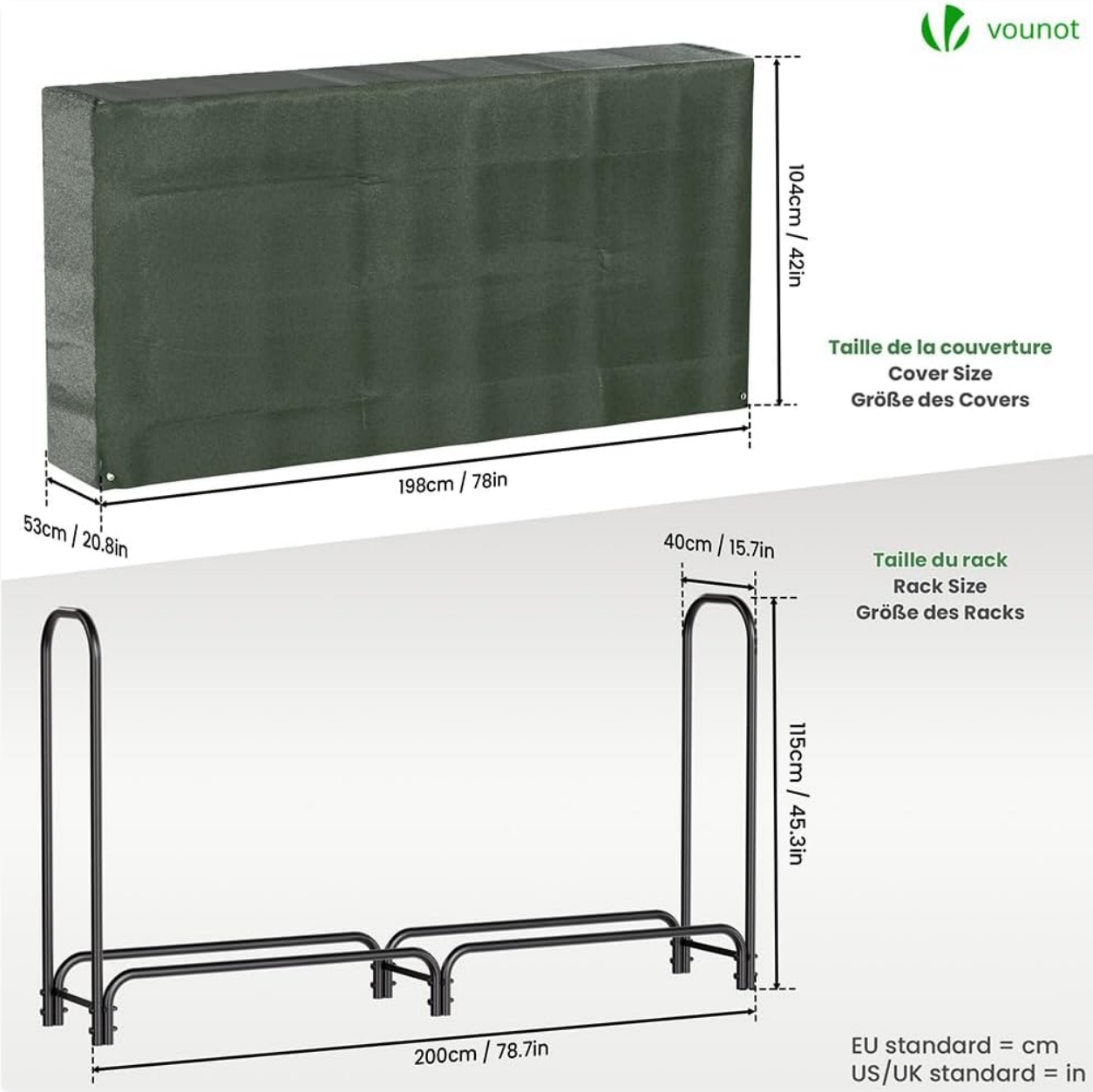
Image: Detailed dimensions of the log rack and its protective cover.
