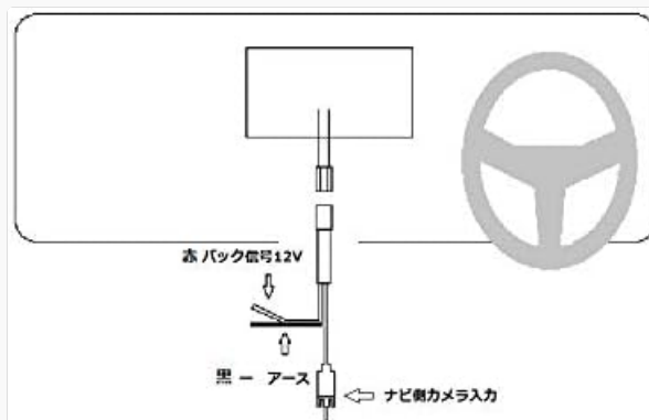
Image: Wiring diagram illustrating the connection points: the 15-pin connector to the camera, the RCA plug to the navigation's camera input, the red wire to the 12V reverse signal, and the black wire to ground.
