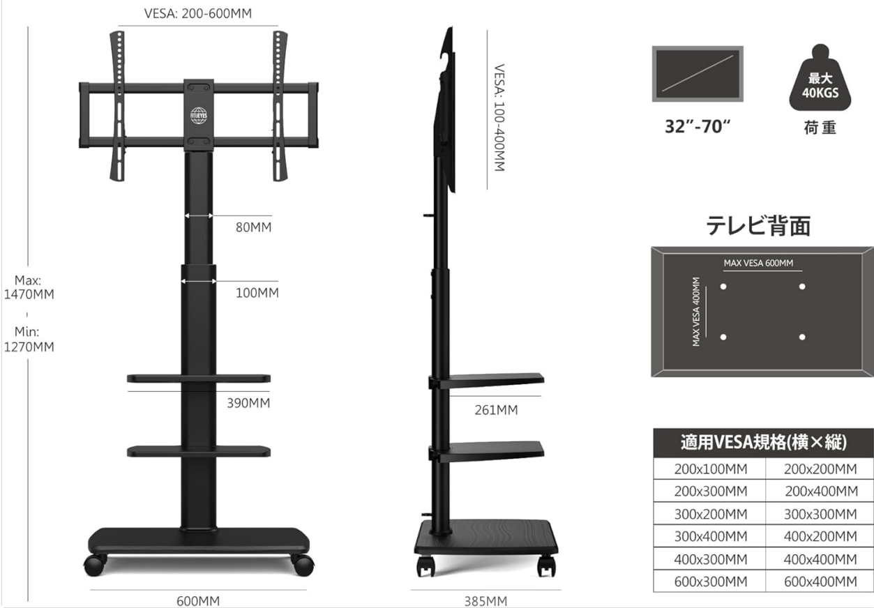
Image 2: Technical diagram illustrating the VESA mounting patterns and overall dimensions of the TV stand.
