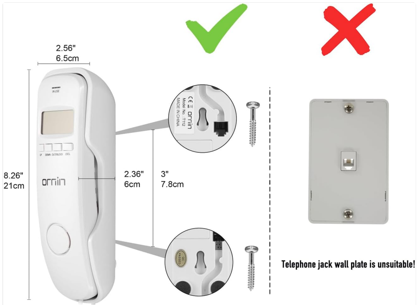
Figure 2: Wall mounting diagram, highlighting the correct method using screws and the incompatibility with standard telephone wall plates.
