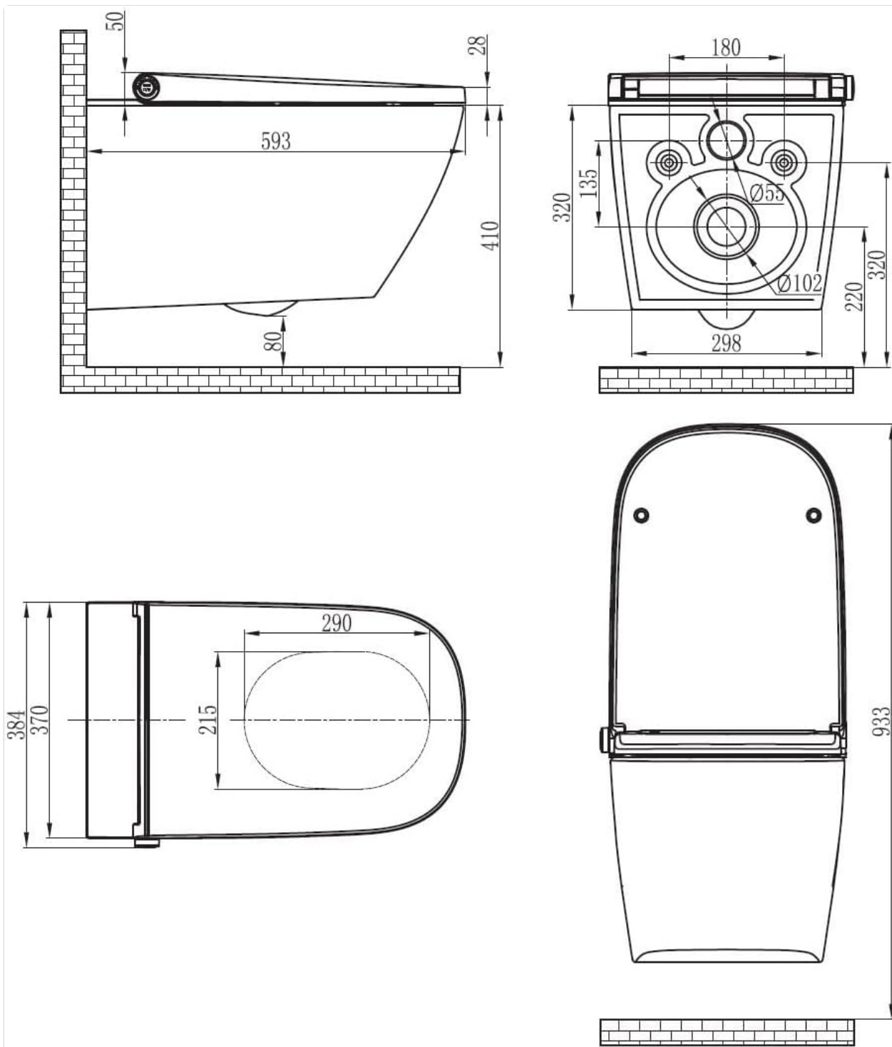
Image 3.1: Technical drawing illustrating the dimensions and installation points for the shower toilet.
