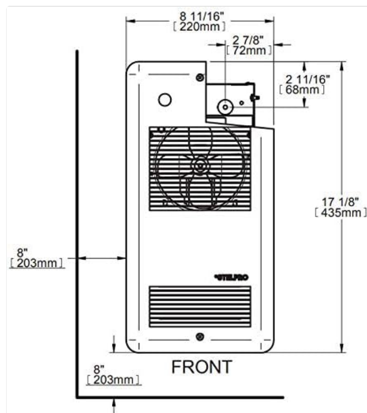
Figure 4: Front dimension diagram.
