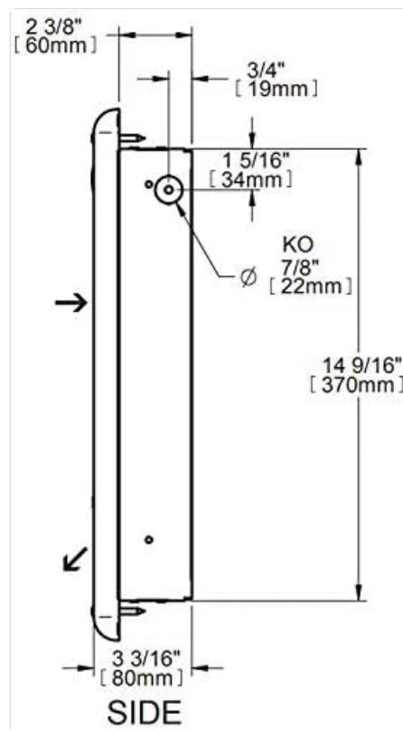
Figure 5: Side dimension diagram.
