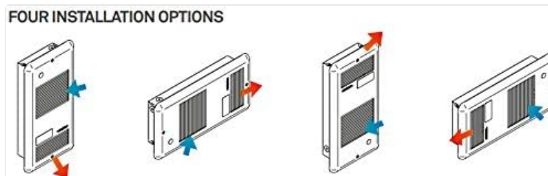
Figure 7: Four installation options for the heater.
