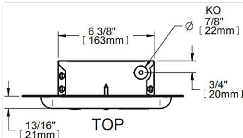
Figure 6: Top dimension diagram.
