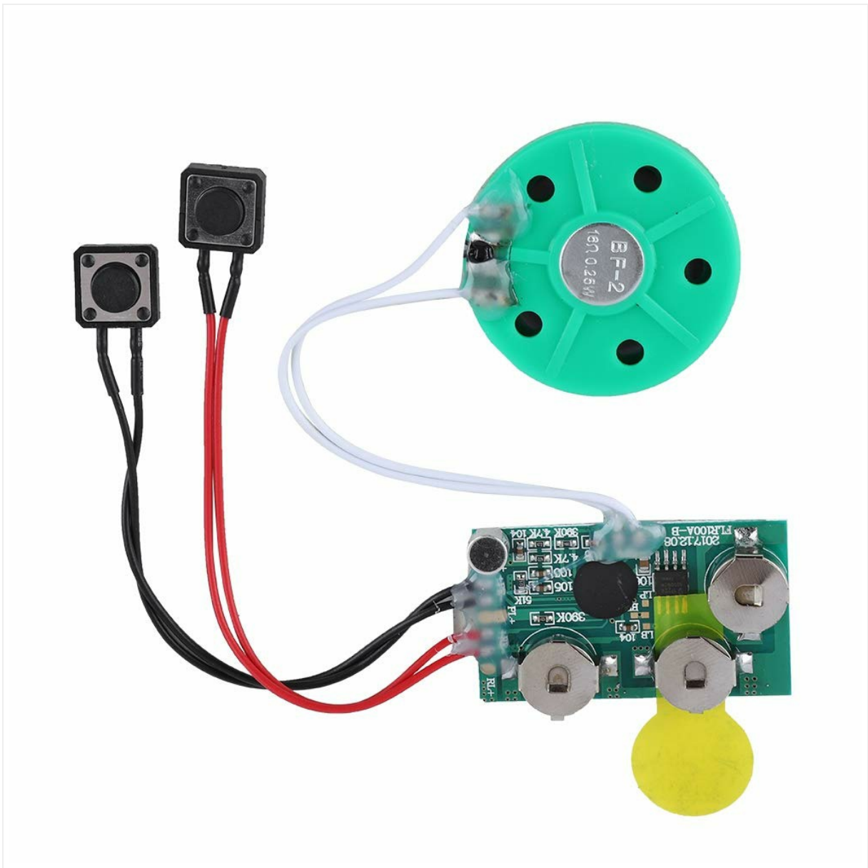
Image 2.1: The voice recording module with the speaker and two control buttons connected via wires.
