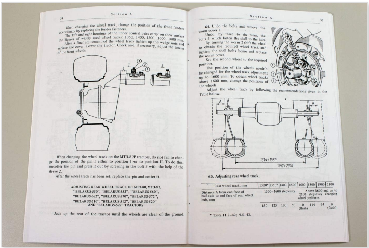
Image: A page from the manual illustrating the process and measurements for adjusting the rear wheel track of the tractor.
