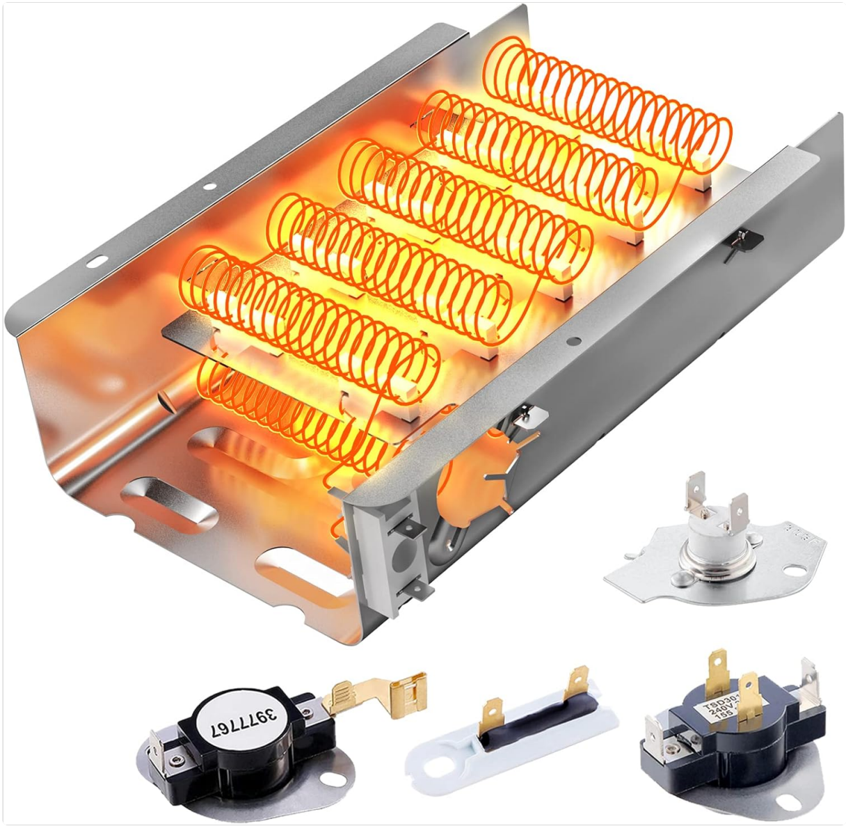
Figure 1: All components included in the SUMNEW 279838 Dryer Heating Element Kit.
