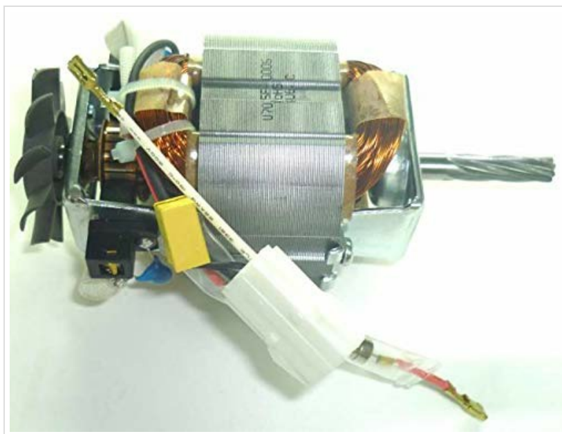
Figure 1: Moulinex Tefal U7035E replacement motor, including carbon brushes and protective fuse.
