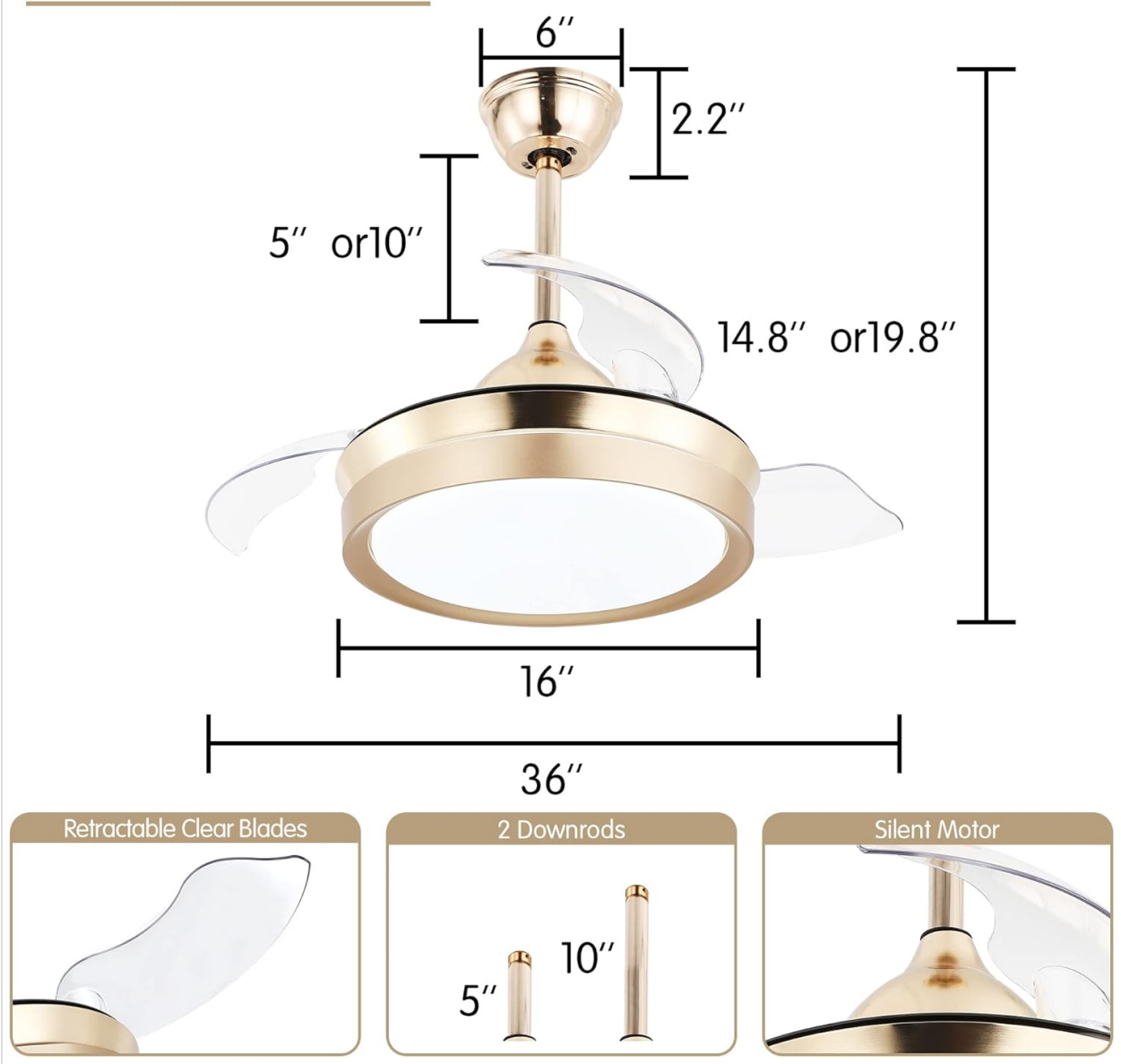
Image: Detailed diagram illustrating the dimensions of the 36-inch ceiling fan, including the canopy, downrods, and overall height and width.
