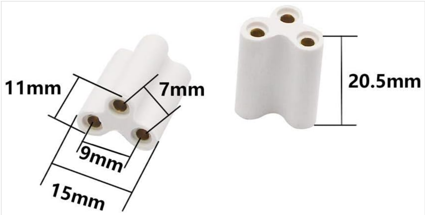
Figure 2: Connector dimensions. The image illustrates the key measurements of the 3-pin connector, including its 20.5mm length.
