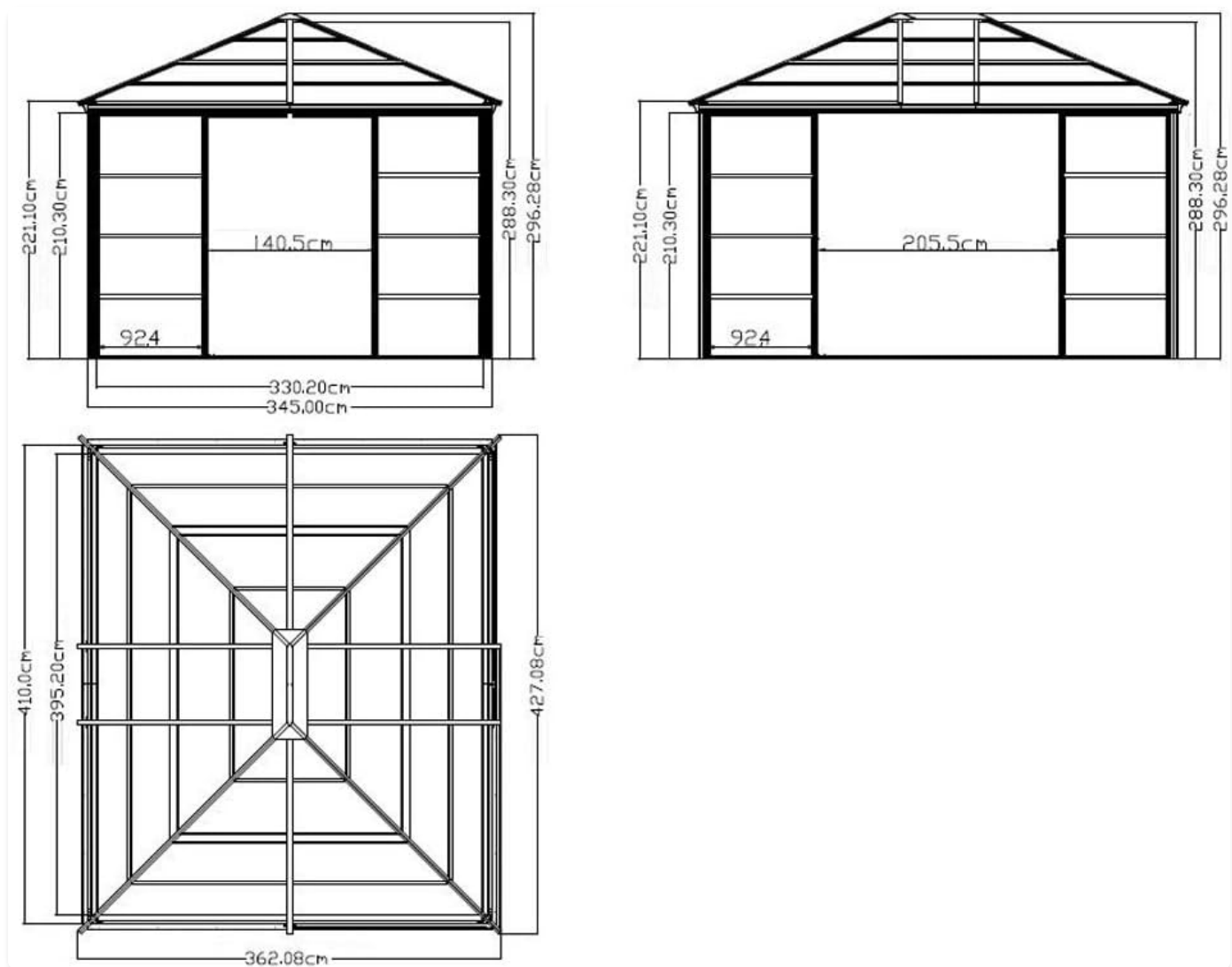
Figure 8.1: Technical dimensions of the Sojag Striano Gazebo.
