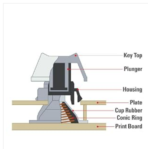
Image: A detailed view of the internal Topre switch mechanism, highlighting its unique design.
