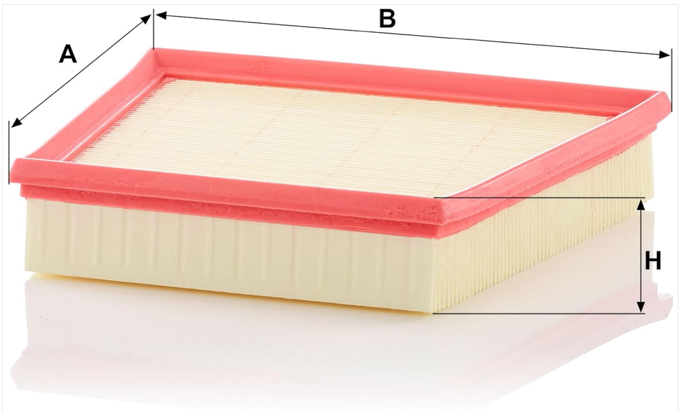
Image: The air filter with labeled dimensions (A, B, H) indicating Length, Width, and Height respectively.
