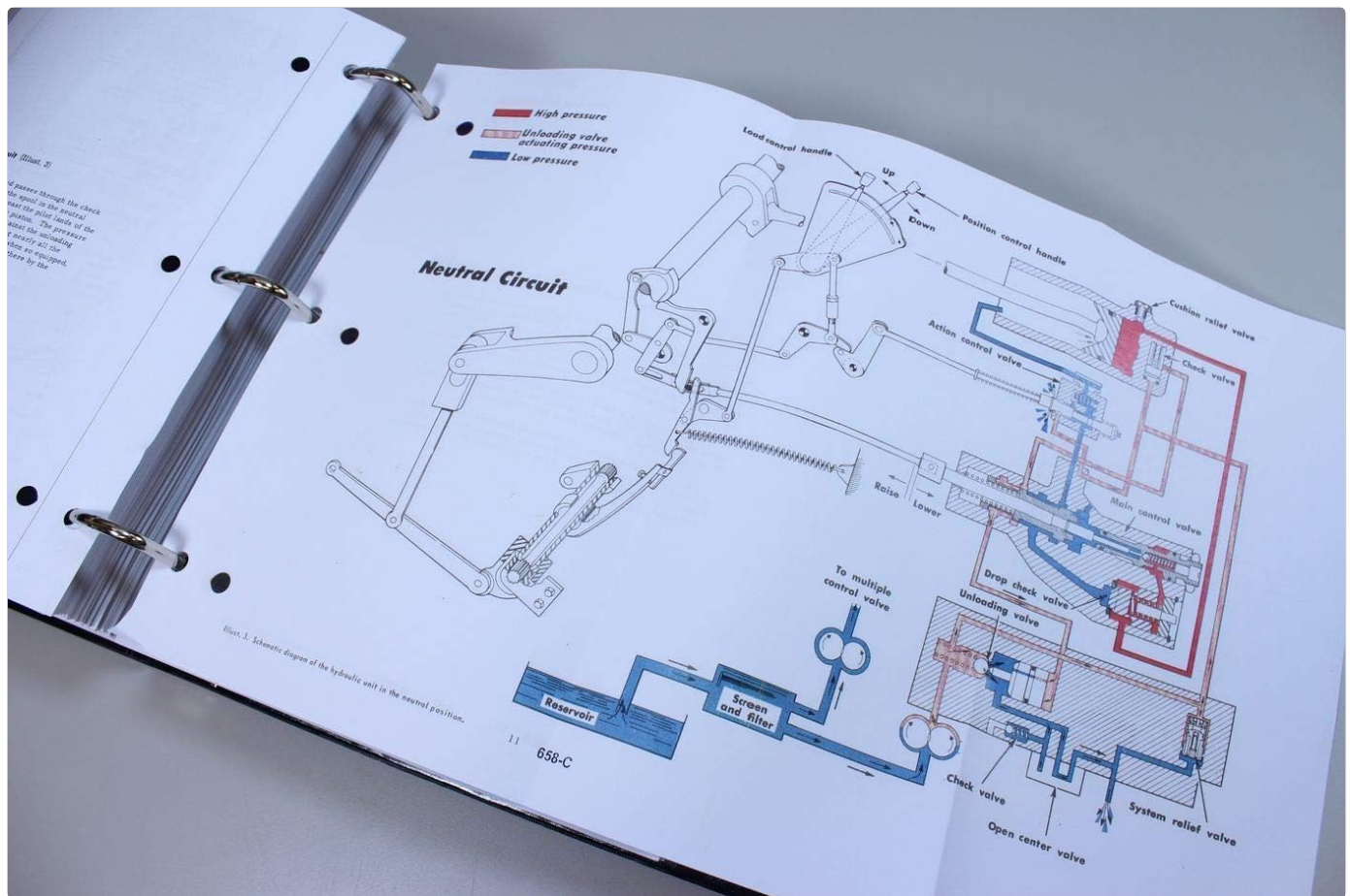
Image: A page from the Service Manual illustrating a 'Neutral Circuit' diagram, detailing the hydraulic control system components and their connections.
