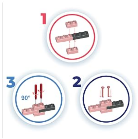
Figure 2: This image provides a three-step visual guide for connecting JEKCA blocks: 1. Align two blocks. 2. Insert the provided pins through the aligned holes. 3. Use the pin driver to turn the pins 90 degrees, locking the blocks securely in place.
