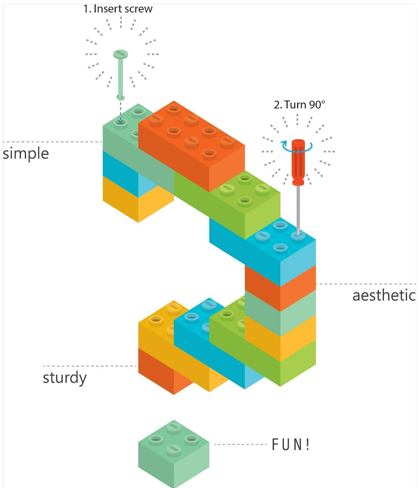
Figure 1: This diagram demonstrates the core mechanism of the JEKCA interlocking system. It shows how a pin is inserted into aligned blocks and then turned 90 degrees with a screwdriver to secure the connection, ensuring a sturdy build.
