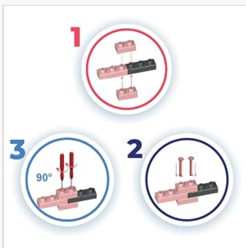
Figure 4.2: Pin Insertion and Rotation. This image details the process: (1) Align blocks, (2) Insert pins, (3) Rotate pins 90 degrees using the pin driver for a secure connection.
