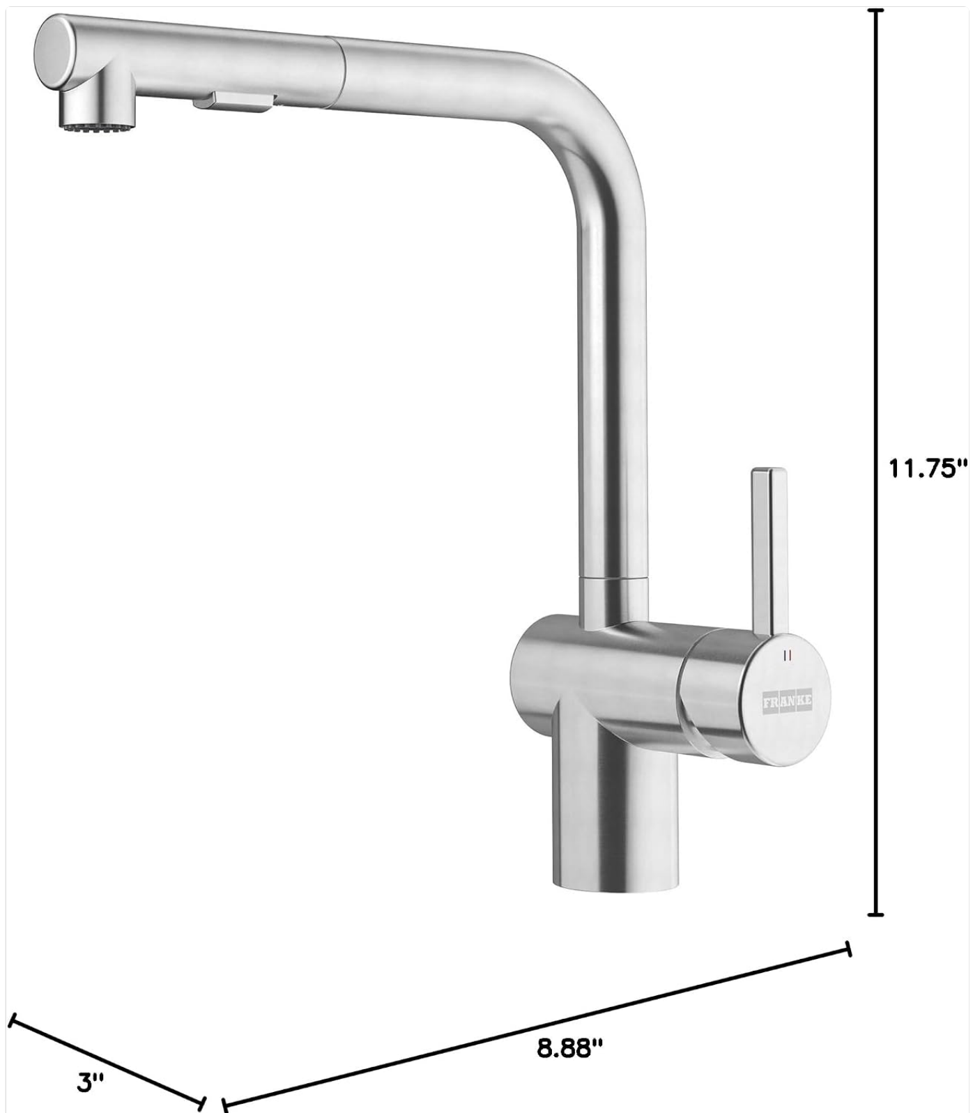
Image: Detailed dimensions of the Franke Atlas NEO faucet, showing its height, depth, and width for installation planning.
