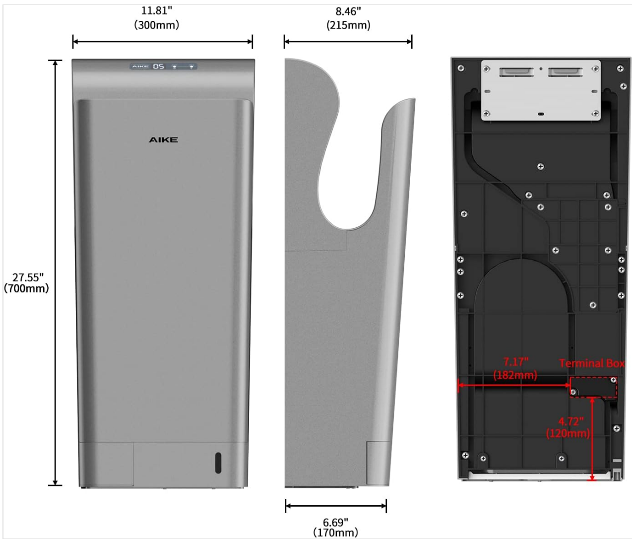
Figure 4.1: Product dimensions of the AIKE AK2030 Hand Dryer.
