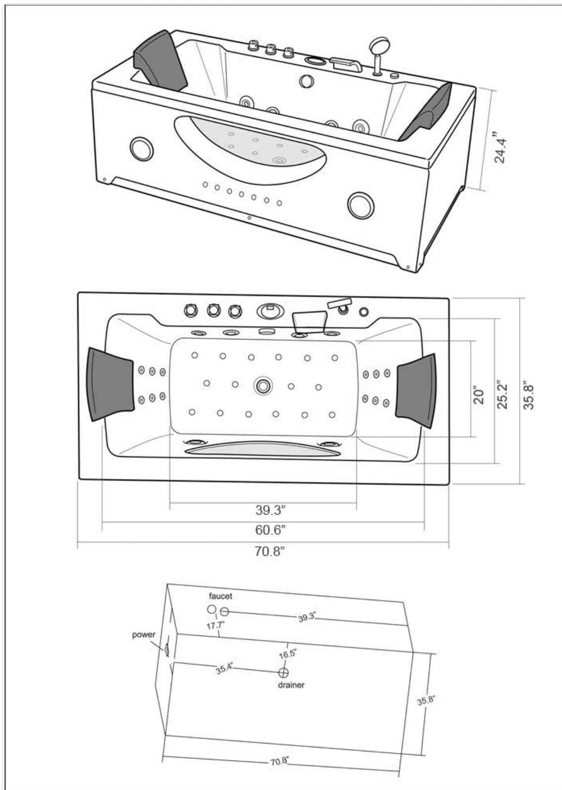
Image 4.1: Technical drawing illustrating the dimensions and layout of the HARMONY bathtub, including power and drain
