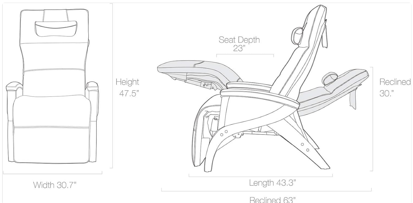
Figure 2: Svago ZGR Newton Recliner in Zero Gravity Position
