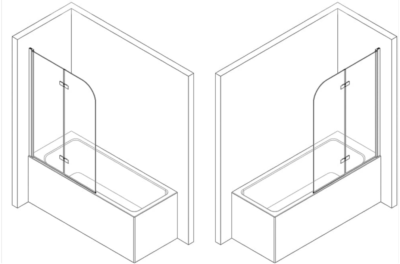
Figure 2: Adjust the installation direction to actual needs (left or right installation).
