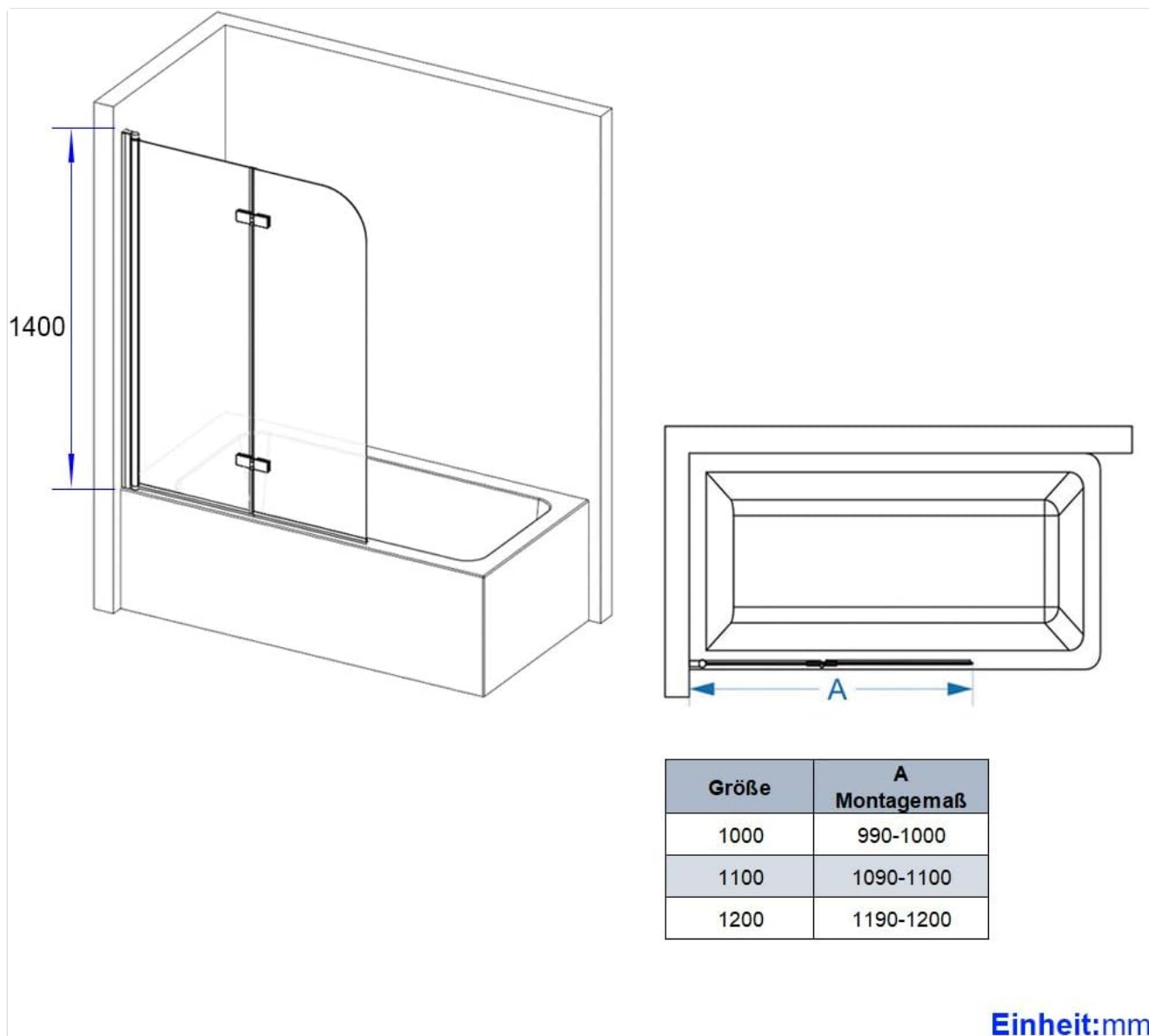
Figure 3: Dimensions and adjustable mounting measurements in millimeters.
