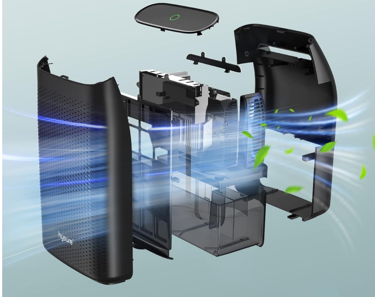
Figure 2.2: Internal components and airflow of the Hysure T8 Plus Dehumidifier.
