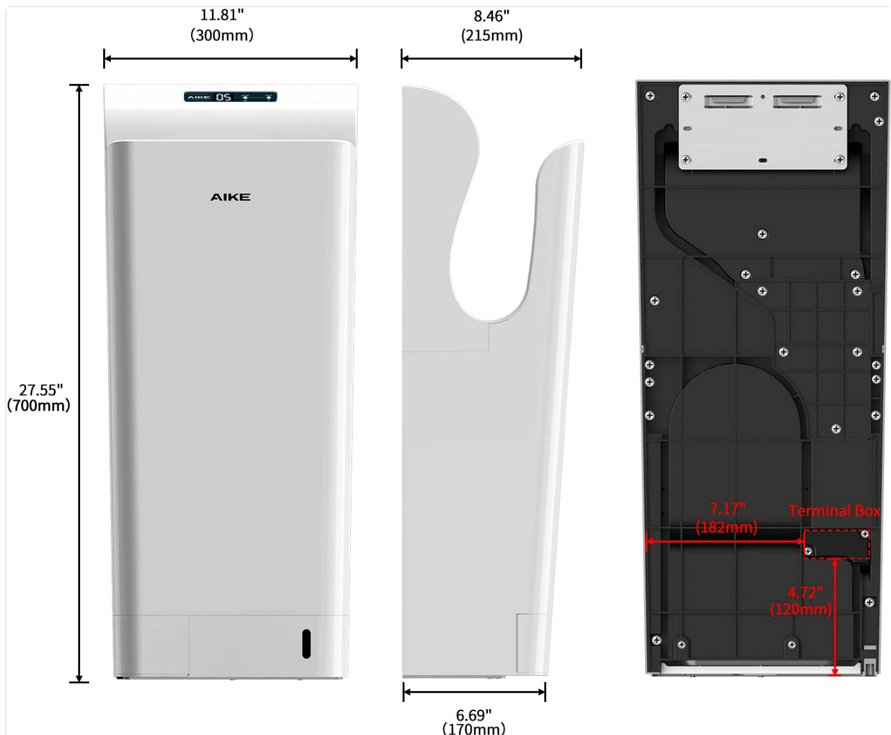
Figure 2: AIKE AK2030 Hand Dryer Dimensions.
