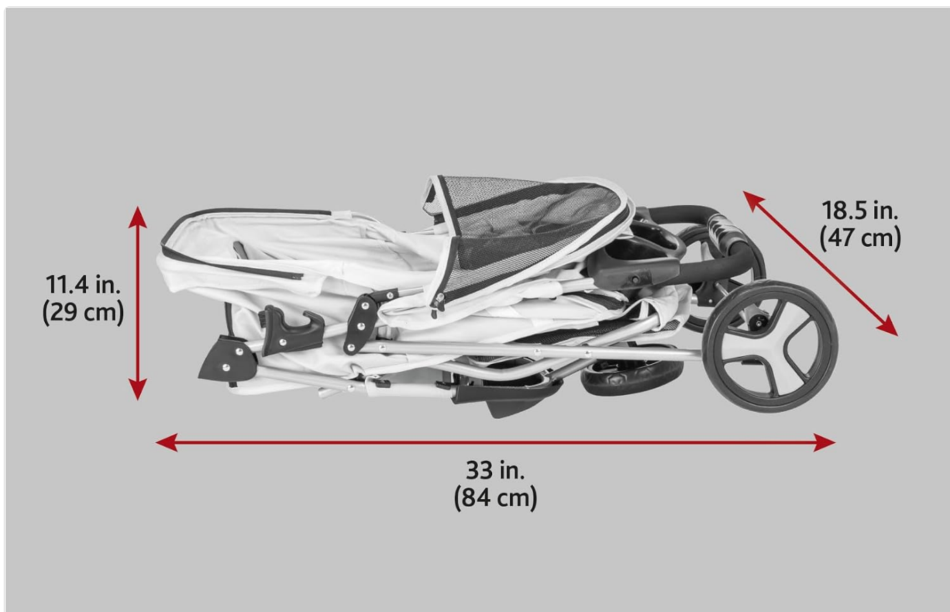
Figure 9: Folded Stroller Dimensions
