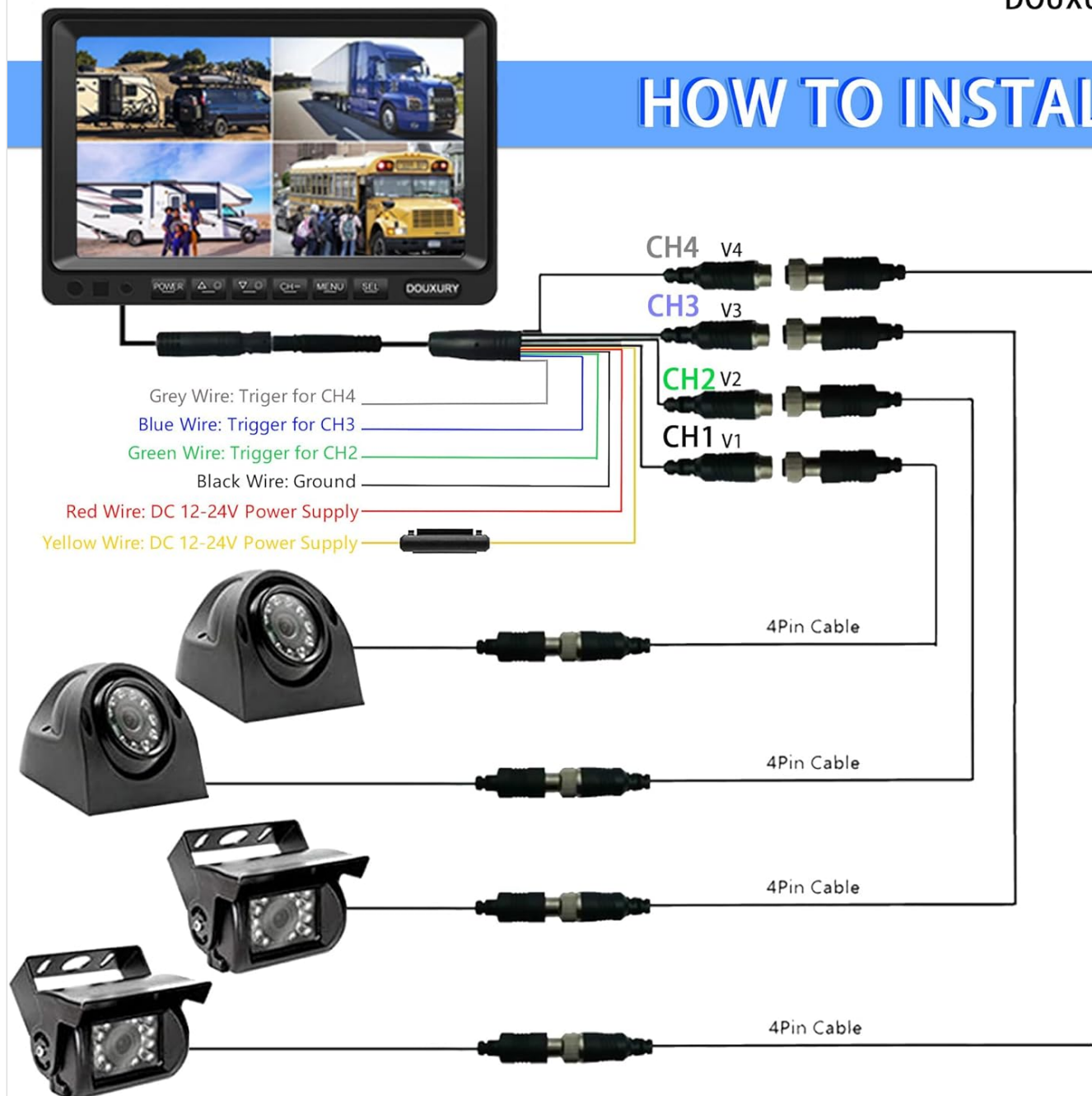
Figure 4: Wiring connections for the monitor and cameras, including power and trigger wires.
