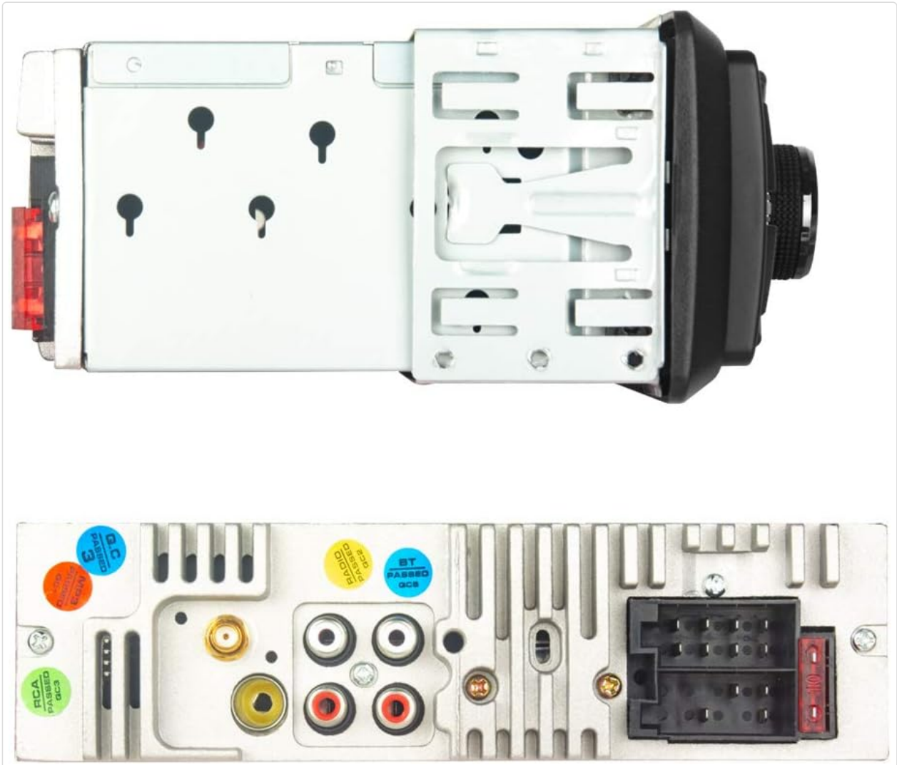
Image 4.3: Rear view of the car stereo, showing the various connectors including the ISO harness port, RCA outputs, and antenna inputs.
