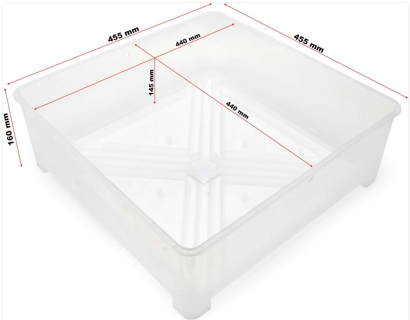
Image 1: Wiltec Replacement Plastic Water Tray. The image displays the clear plastic tray with key dimensions labeled: 455 mm (length), 455 mm (width), 160 mm (height), and internal dimensions of 440 mm by 440 mm with a depth of 145 mm.
