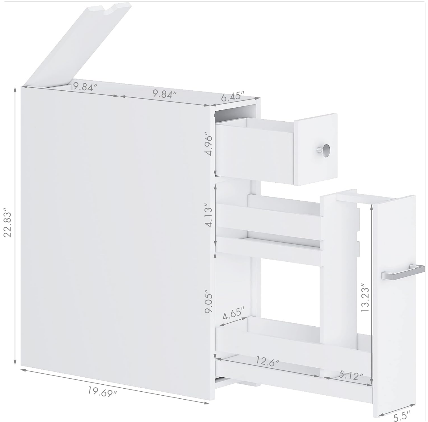
Figure 2: Detailed dimensions of the cabinet and its internal compartments.
