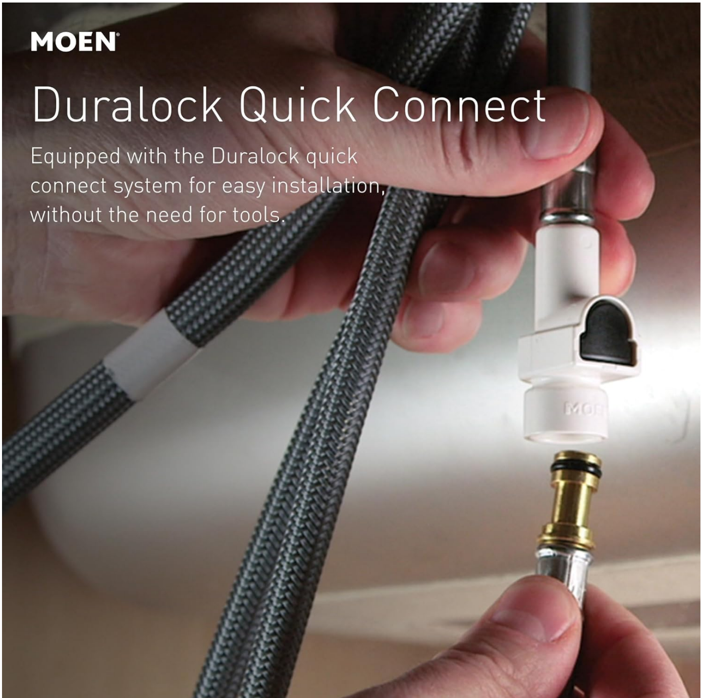
Figure 5.2: Duralock Quick Connect System. This image demonstrates the easy, tool-free connection of the faucet's supply lines using the Duralock system.
