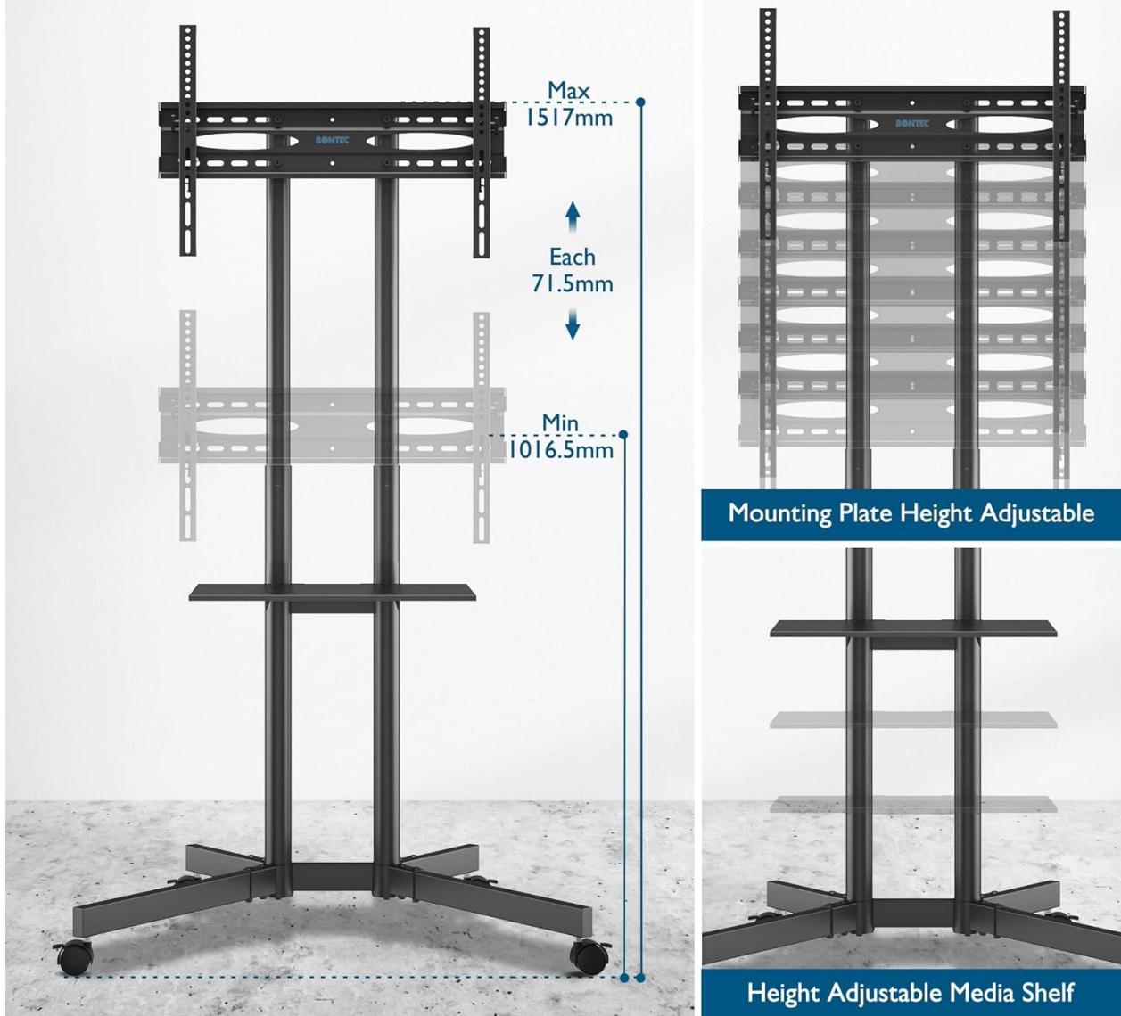
Image: Diagram illustrating the height adjustment range for the TV mounting plate (Min 1016.5mm, Max 1517mm) and the adjustable media shelf.
