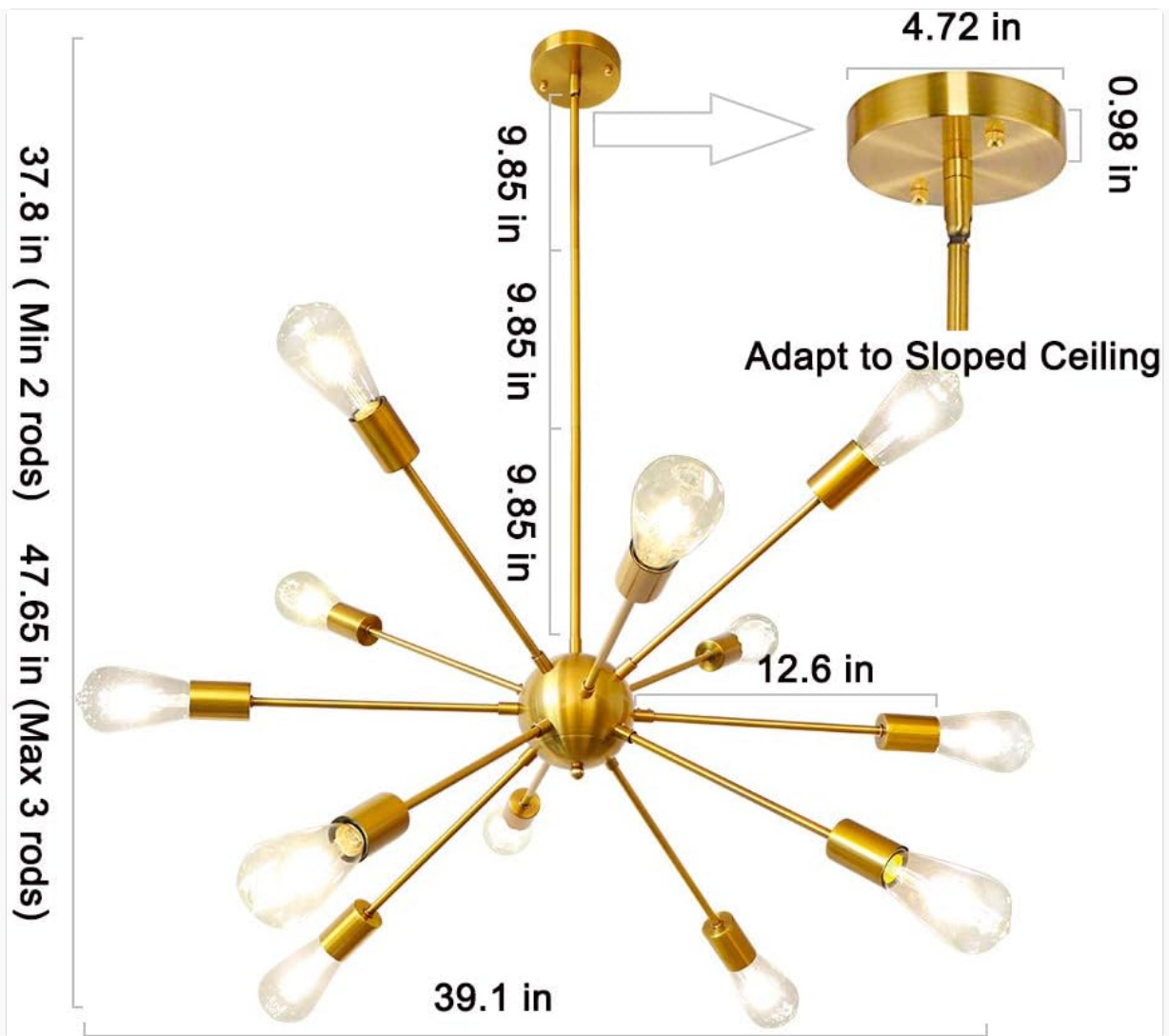
Image: Diagram illustrating the adjustable height feature using three extension rods and how the canopy adapts to sloped ceilings.
