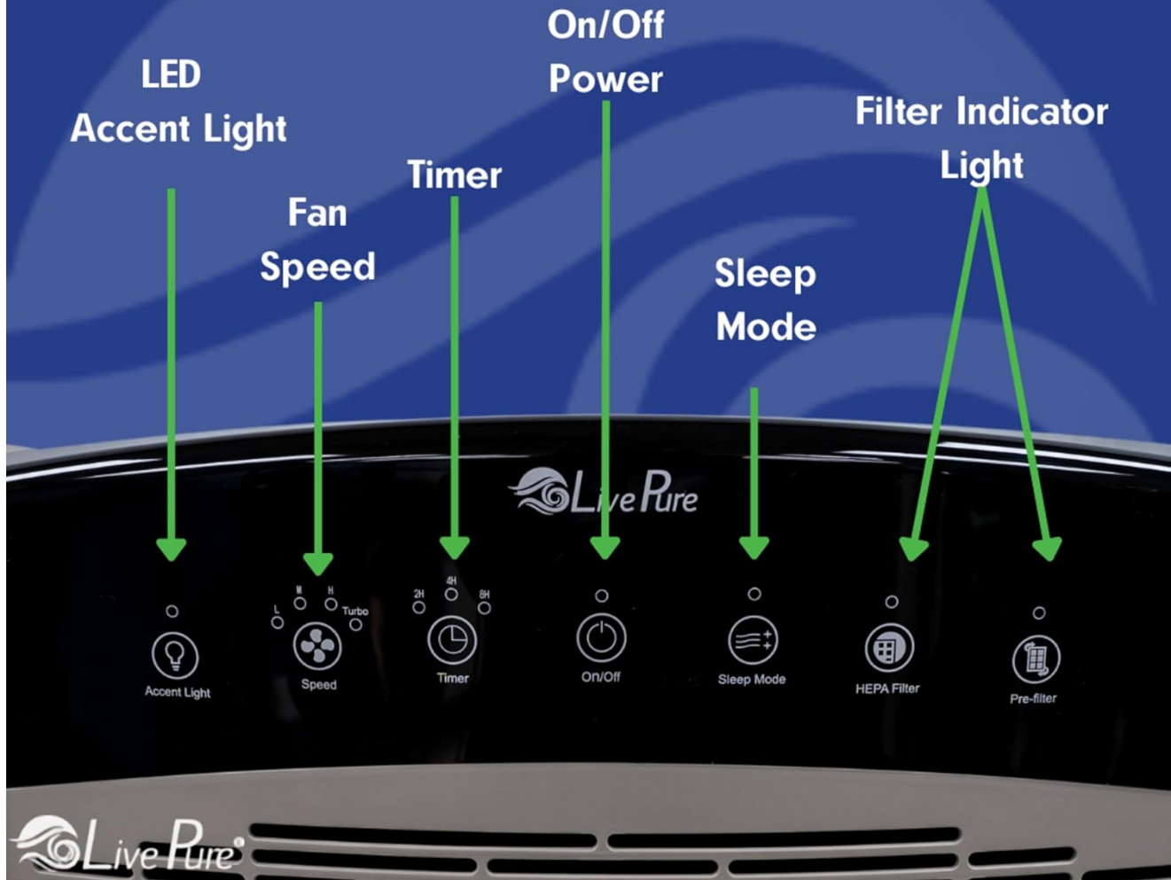
Figure 5: Close-up of the control panel, highlighting the LED Accent Light, Fan Speed, Timer, On/Off Power, Sleep Mode, HEPA Filter indicator, and Pre-filter indicator.
