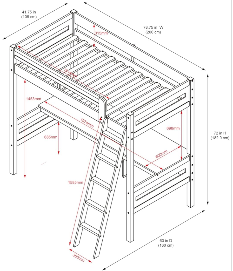
Image: A detailed dimensional drawing of the DHP Harlan Loft Bed, illustrating its overall dimensions and key measurements for planning placement and assembly.
