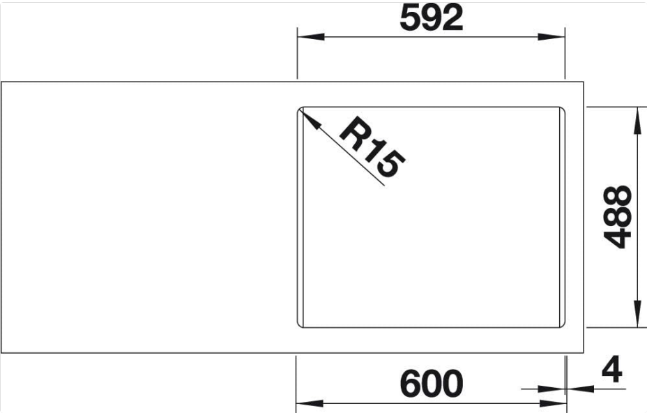
Image 2.4: Countertop cutout diagram for the BLANCO PALONA 6 sink, indicating a cutout width of 592mm and depth of 488mm, with R15 corner radii.
