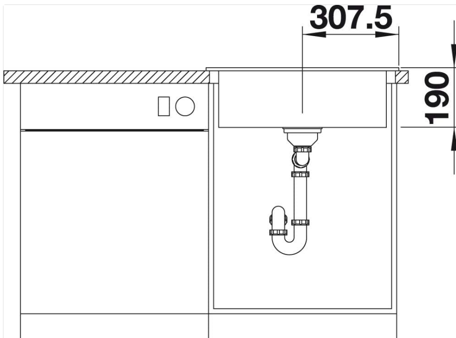
Image 2.2: Side view installation diagram of the BLANCO PALONA 6 sink, illustrating the sink's depth (190mm) and clearance required for the drain fitting under a countertop.
