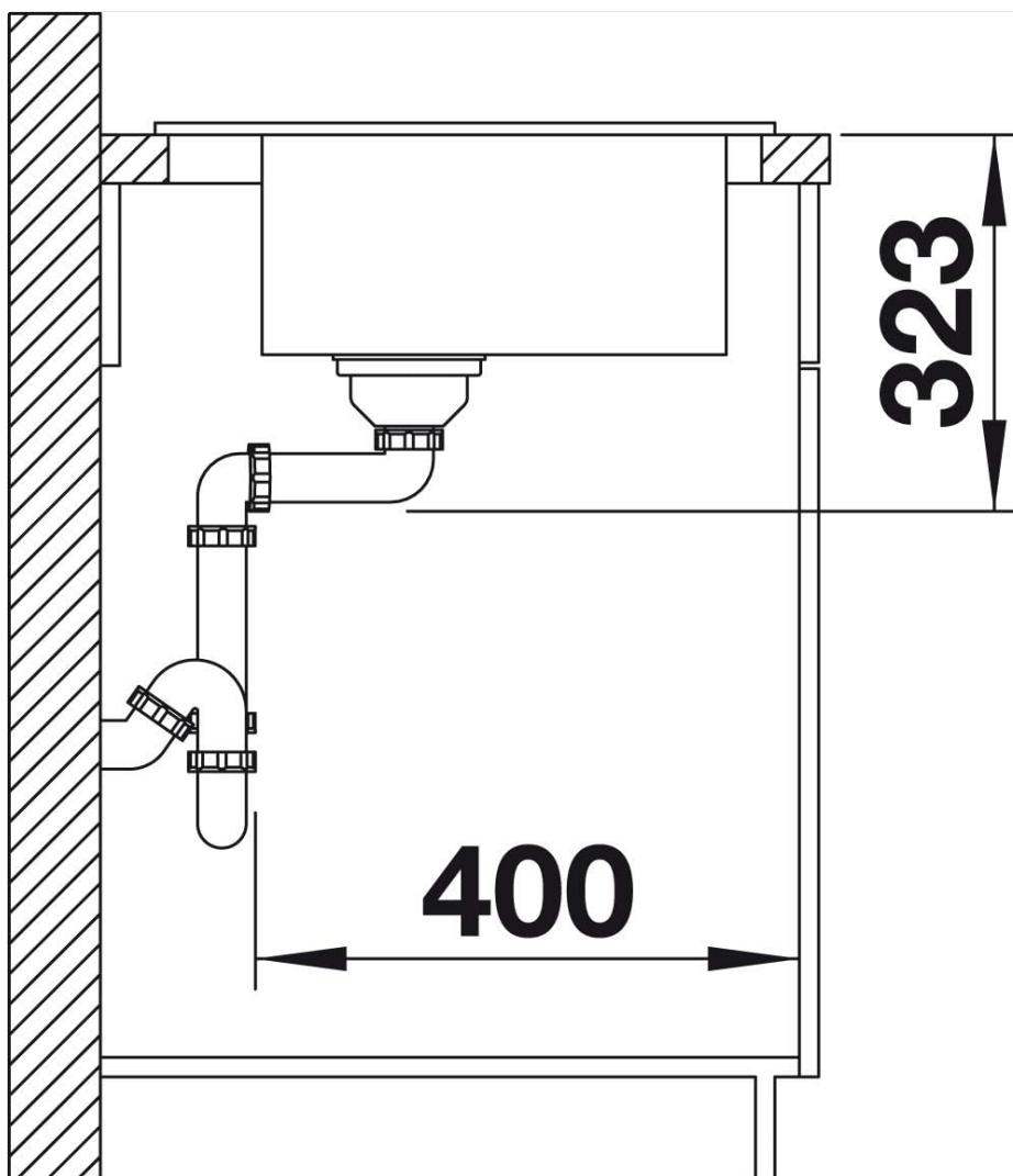
Image 2.3: Detailed side view diagram showing the total depth of the BLANCO PALONA 6 sink (323mm from top of counter to bottom of drain pipe) and the required undercounter space (400mm).
