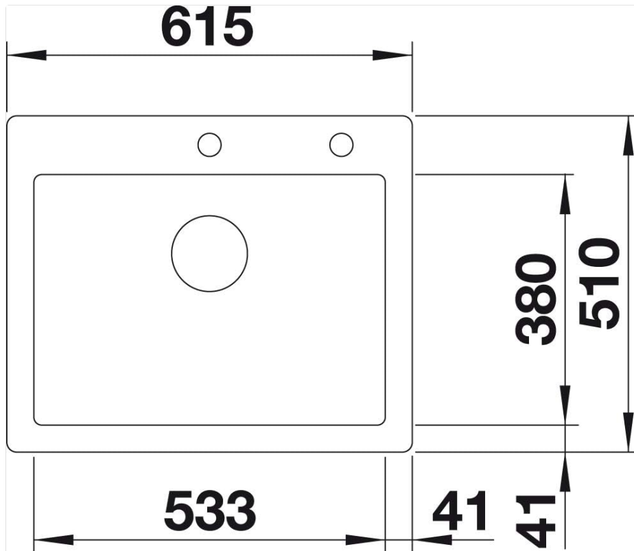
Image 2.1: Top-down dimension diagram of the BLANCO PALONA 6 sink, showing overall width (615mm) and depth (510mm), and bowl dimensions (533mm width, 380mm depth).
