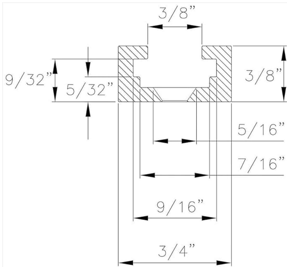
Figure 7: Detailed cross-sectional view of the T-track, providing additional internal and external measurements.
