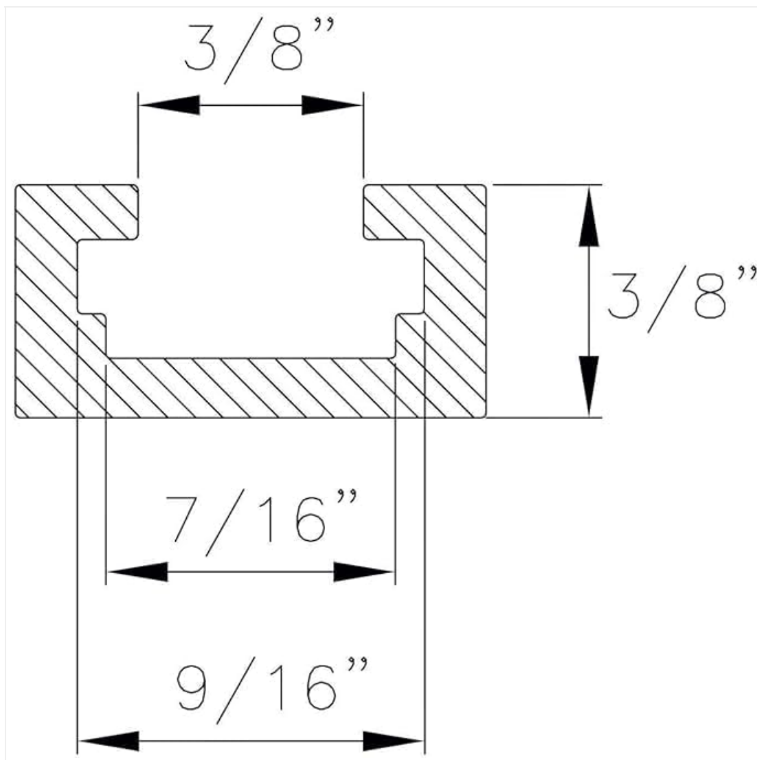
Figure 6: Cross-sectional dimensions of the T-track, indicating key measurements for compatibility.
