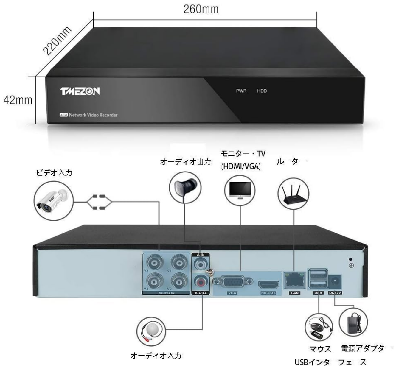
Figure 4.1: DVR Connection Ports
